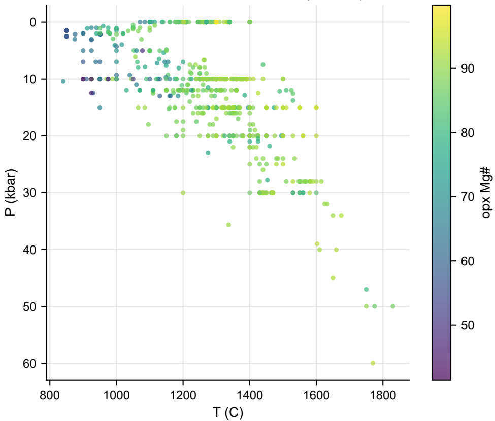
opx-liq experimental distribution (n = 600)
