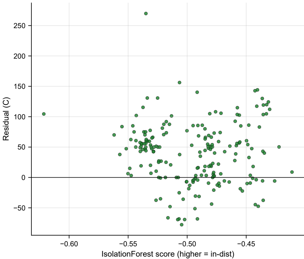
T_C residual vs OOD score
