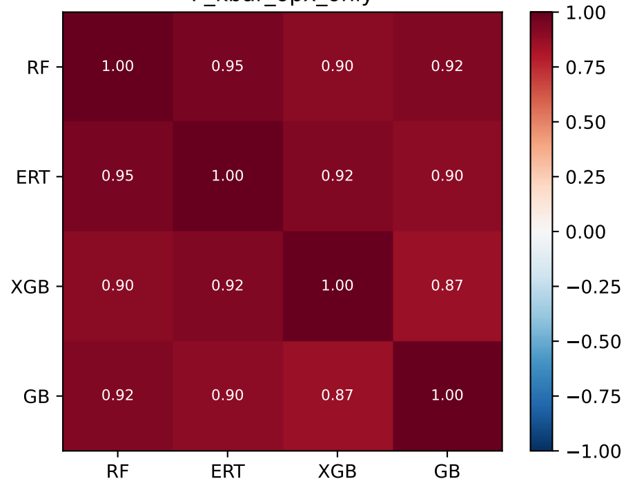
P_kbar_opx_only
