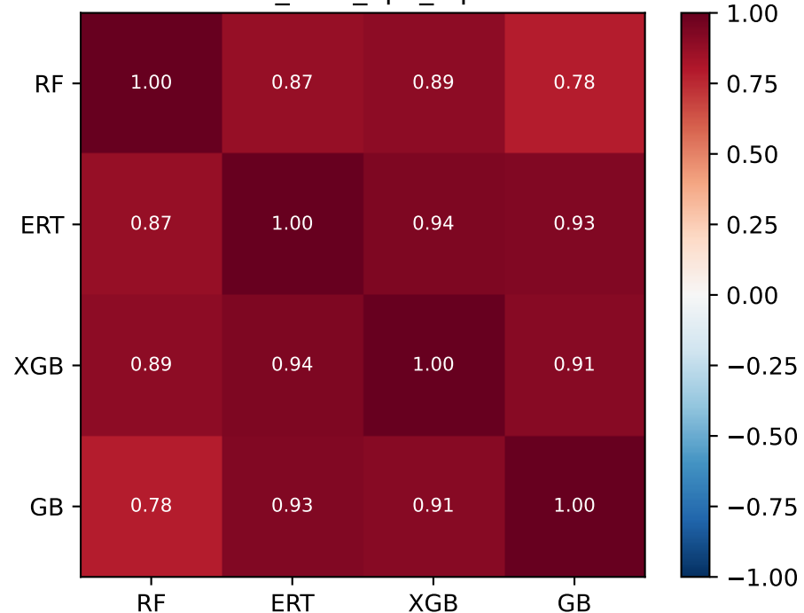
P_kbar_opx_only
