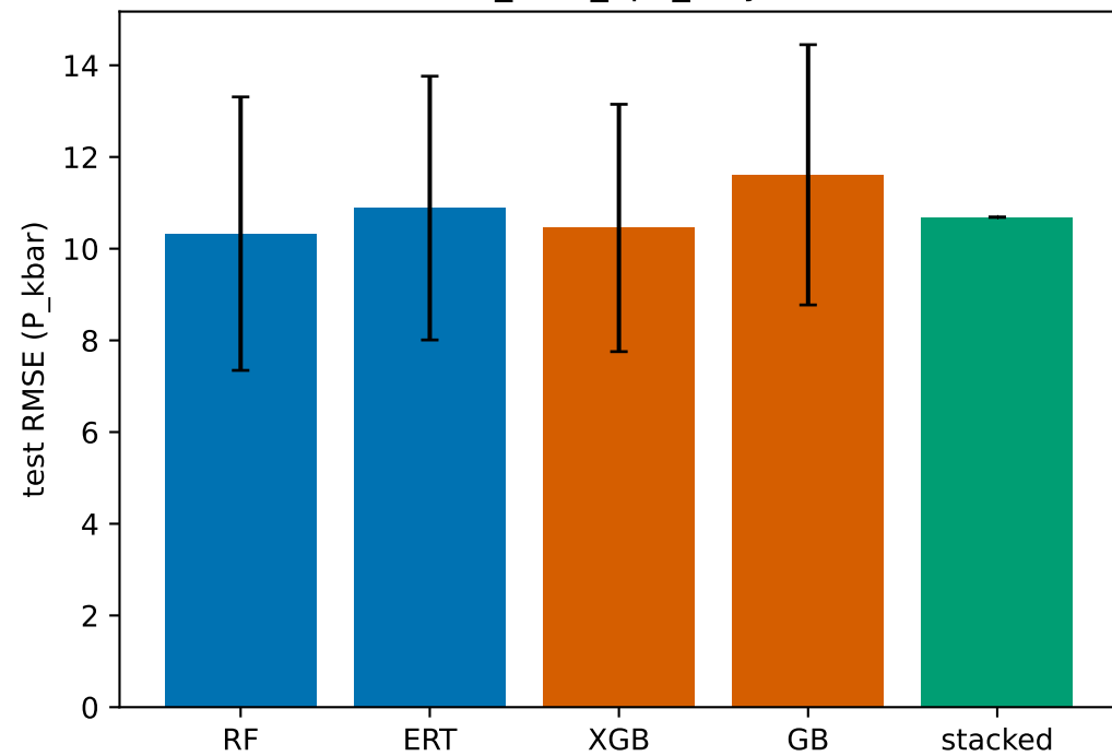
P_kbar_opx_only
