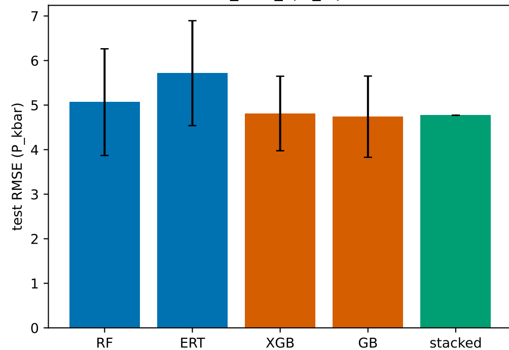
P_kbar_opx_only
