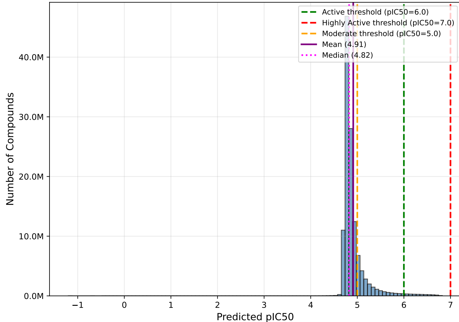
pIC50 Distribution - Full Range
