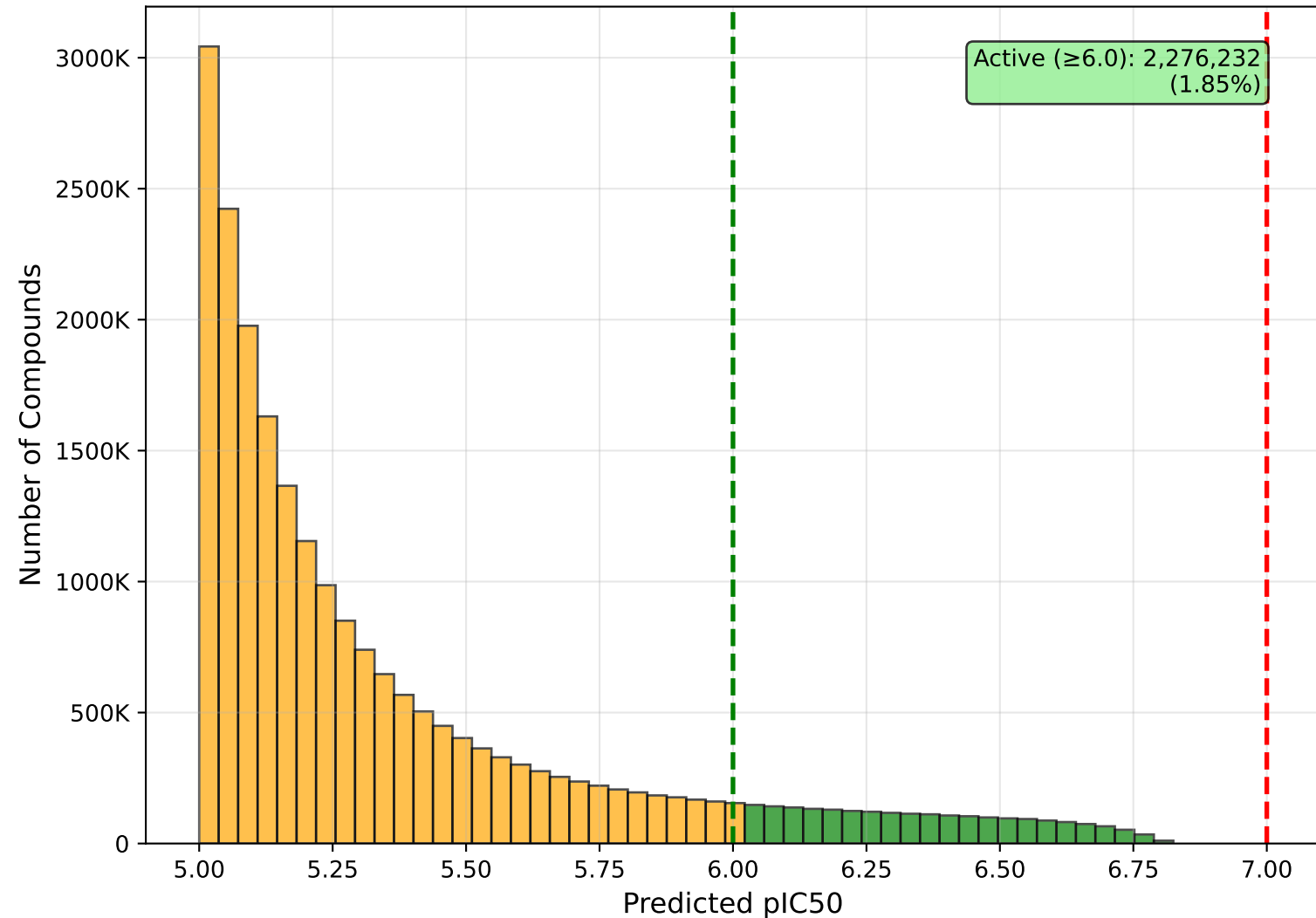
pIC50 Distribution - Active Region (pIC50 ≥ 5.0)
