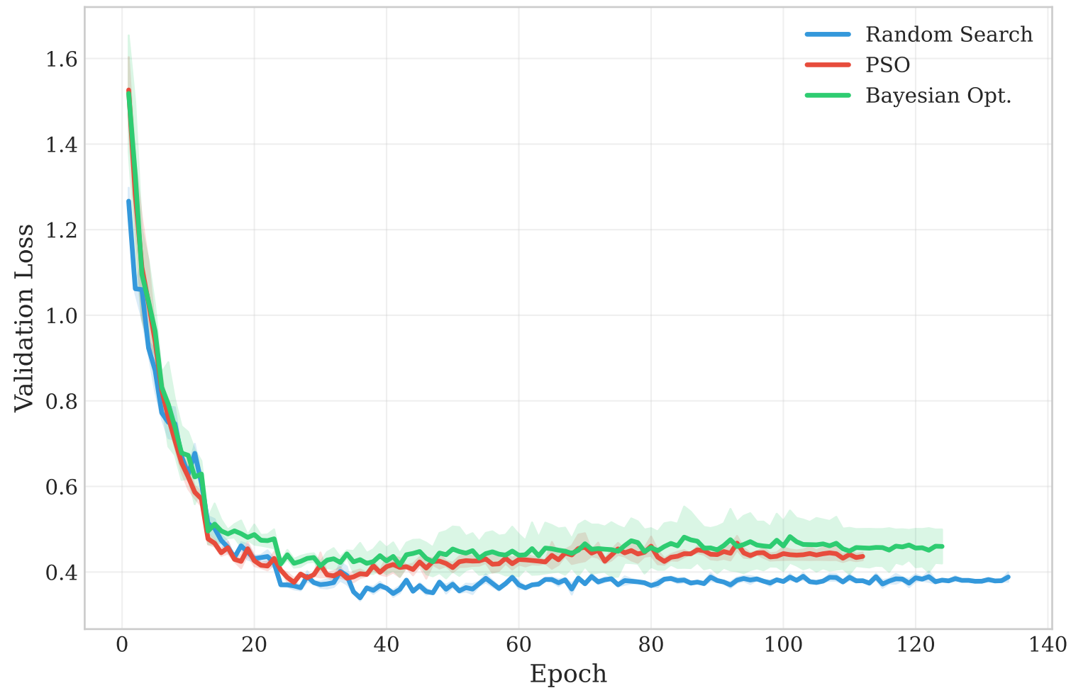
Validation Loss (mean \pm std)
