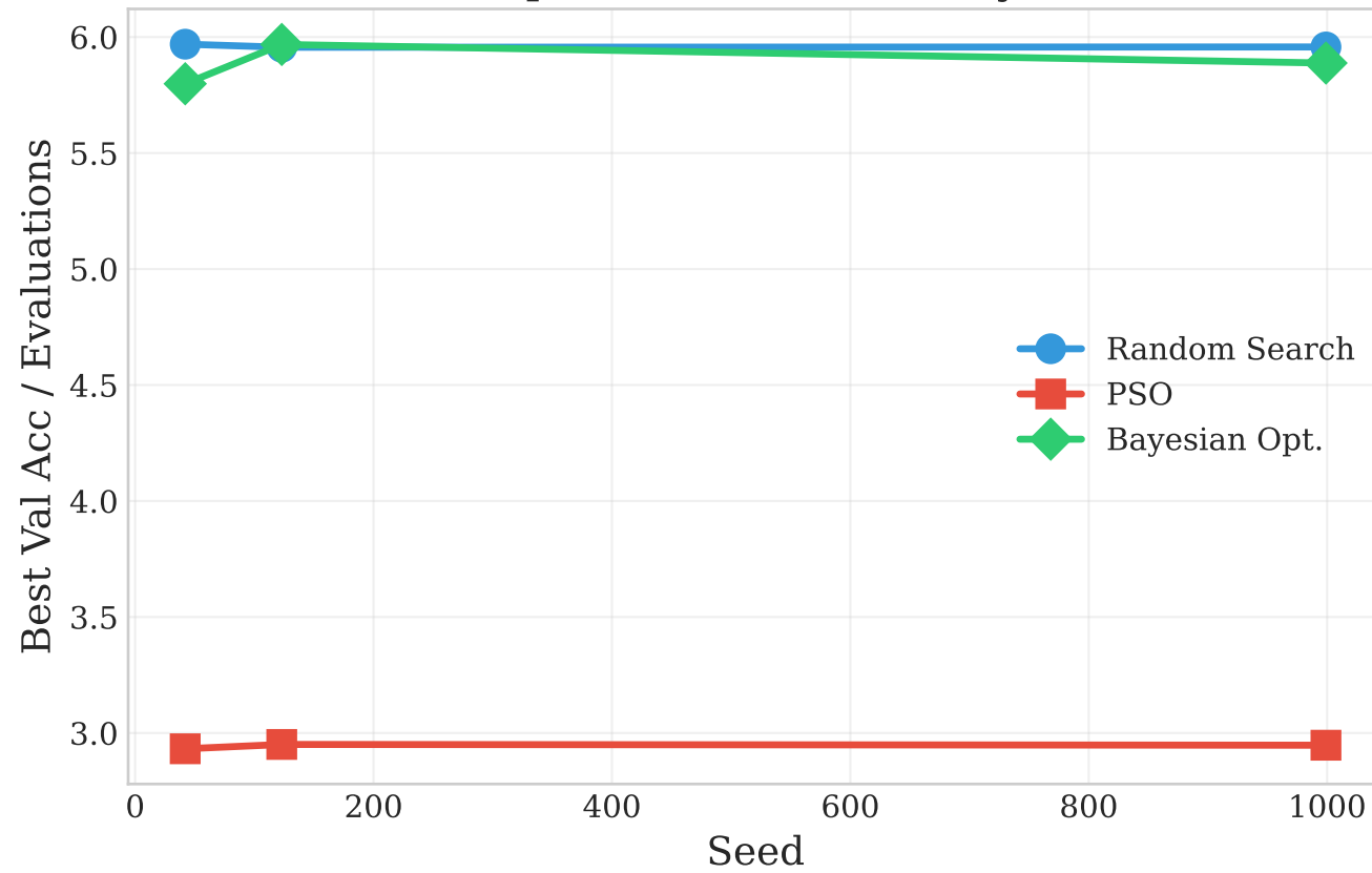
Optimization Efficiency
