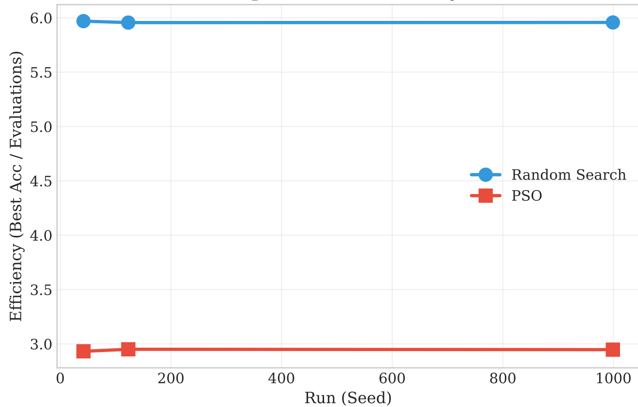
Optimization Efficiency
