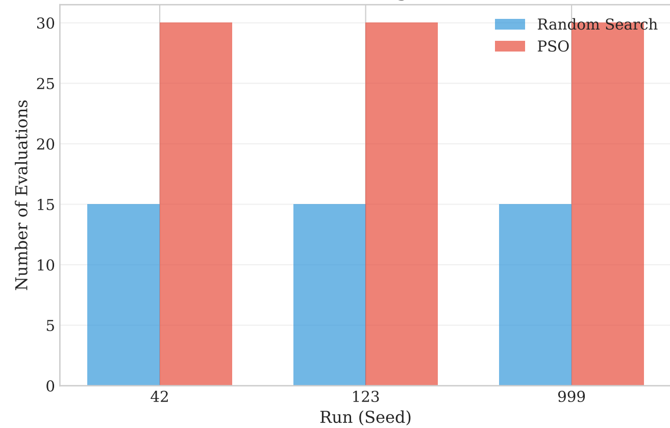
Optimization Efficiency
