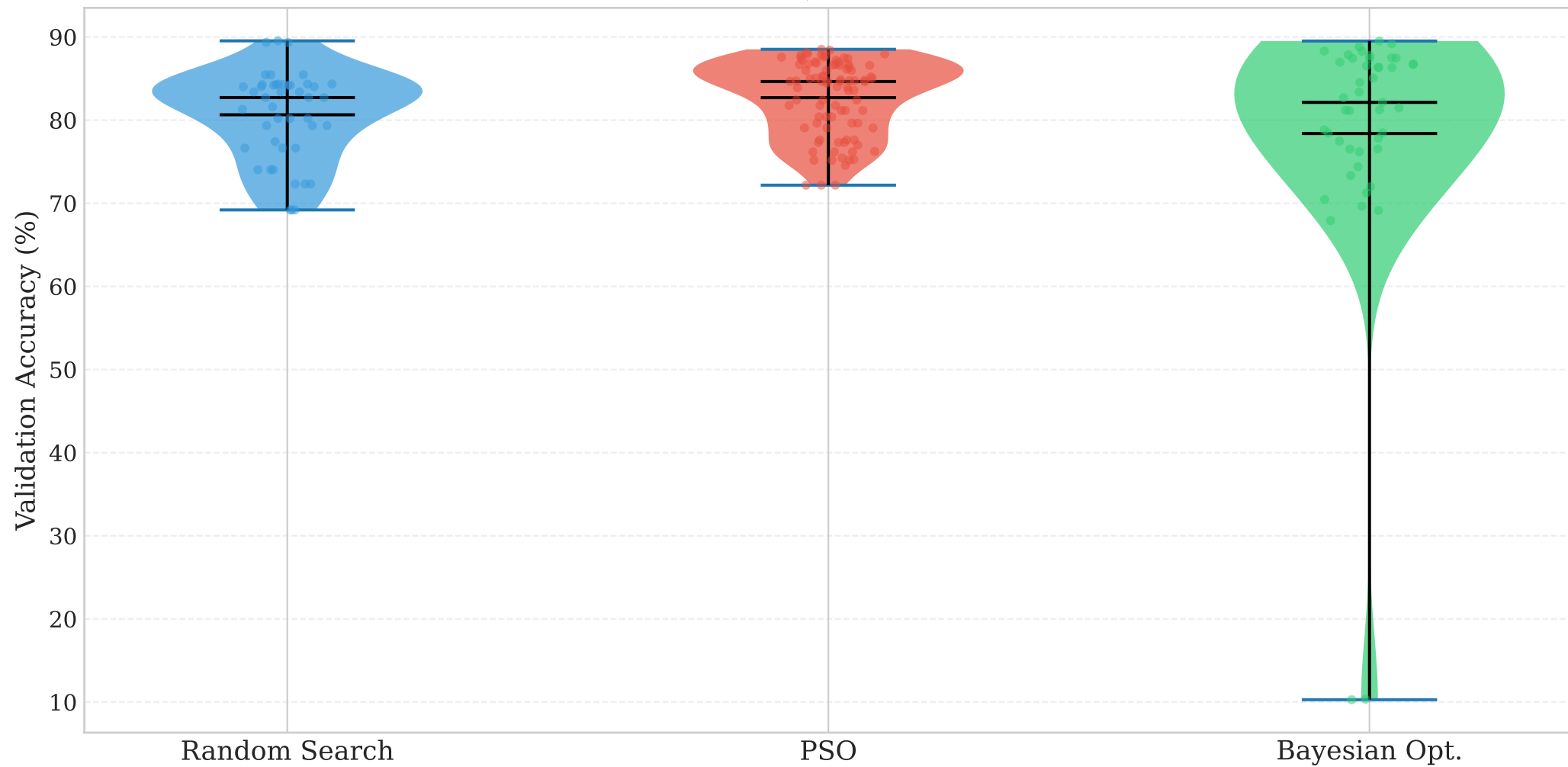
Distribution of ALL Trial Accuracies per Method (mean=◆, median=—)
