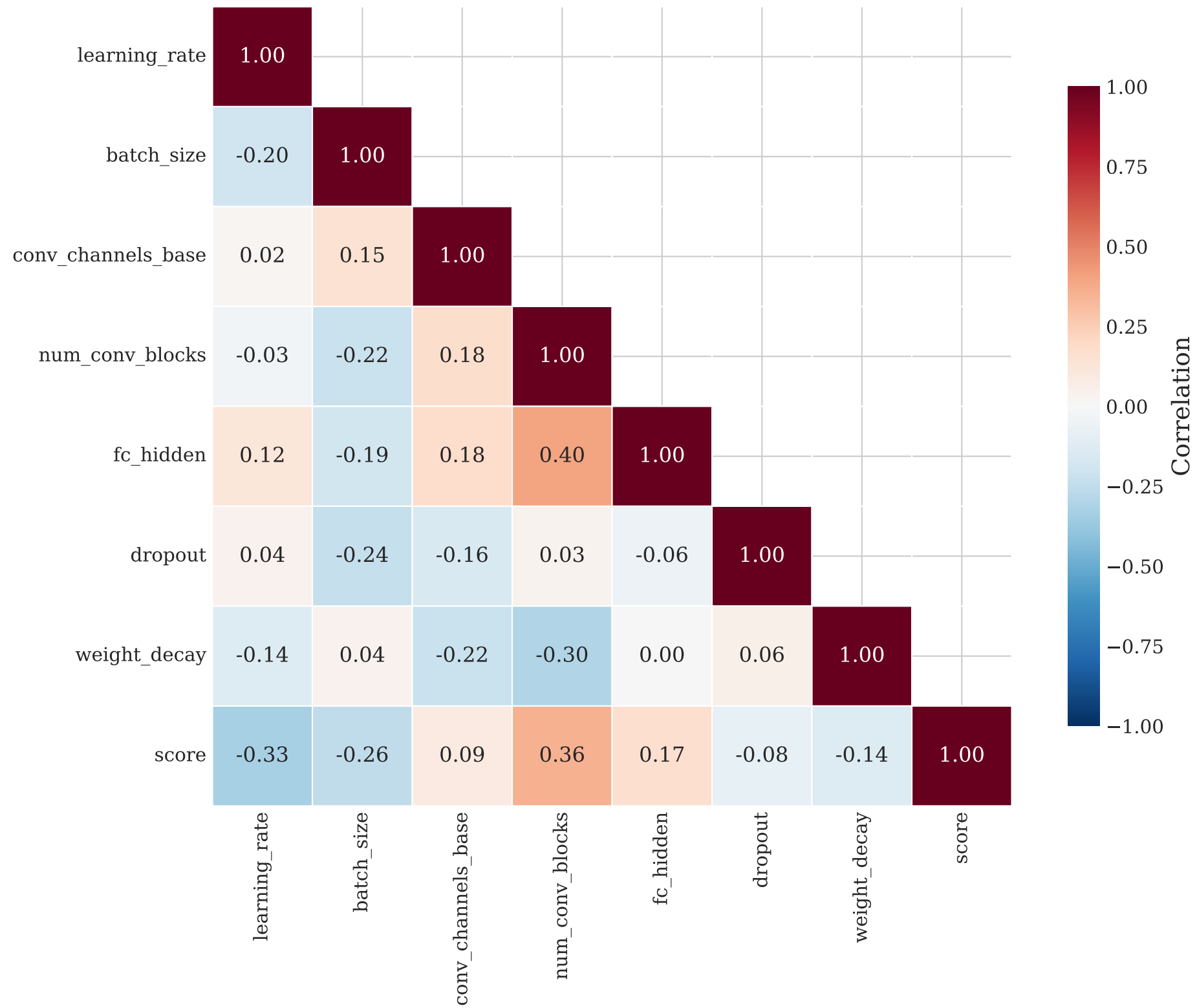
Hyperparameter Correlation Matrix (All methods combined)
