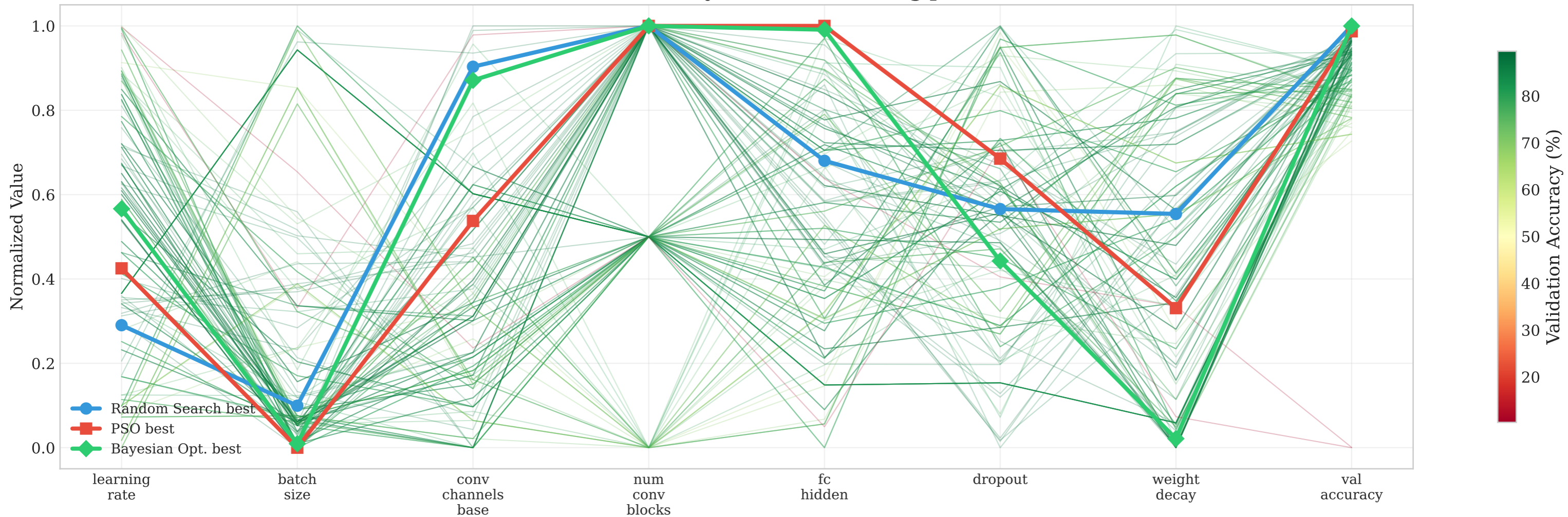
Parallel Coordinates — Search Space Exploration (Color = validation accuracy, bold = best config per method)
