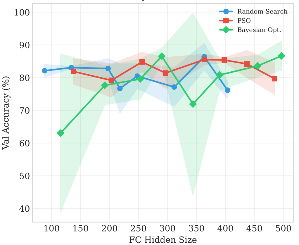
Sensitivity: FC Hidden Size
