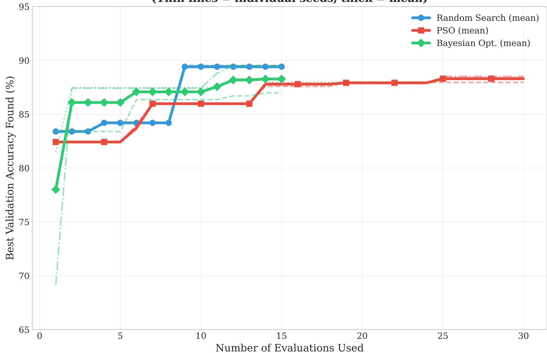
Cost-Benefit Frontier (Thin lines = individual seeds, thick = mean)
