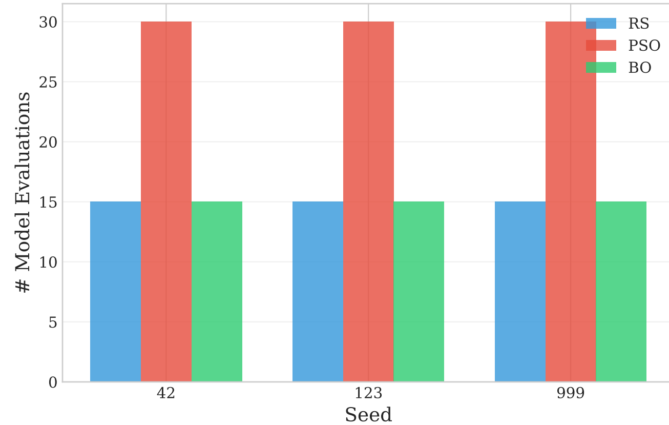
Optimization Efficiency
