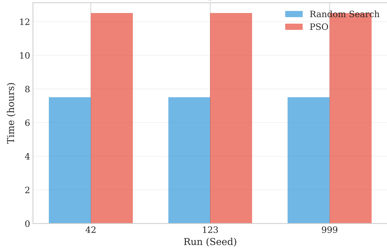
Convergence Speed
