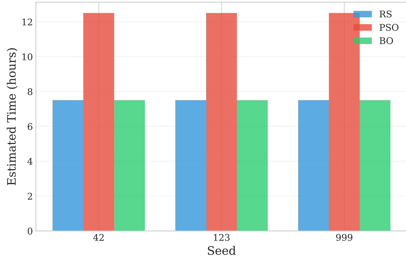
Convergence Speed
