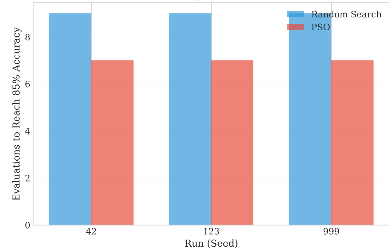
Convergence Speed
