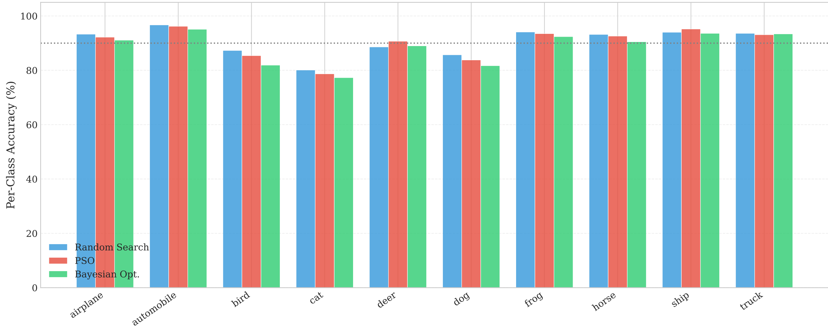
Per-Class Accuracy Comparison — RS vs PSO vs Bayesian Opt. (Seed 42)
