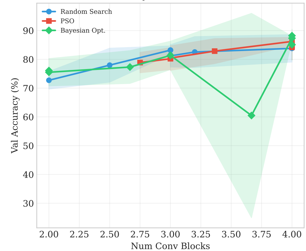
Sensitivity: Num Conv Blocks
