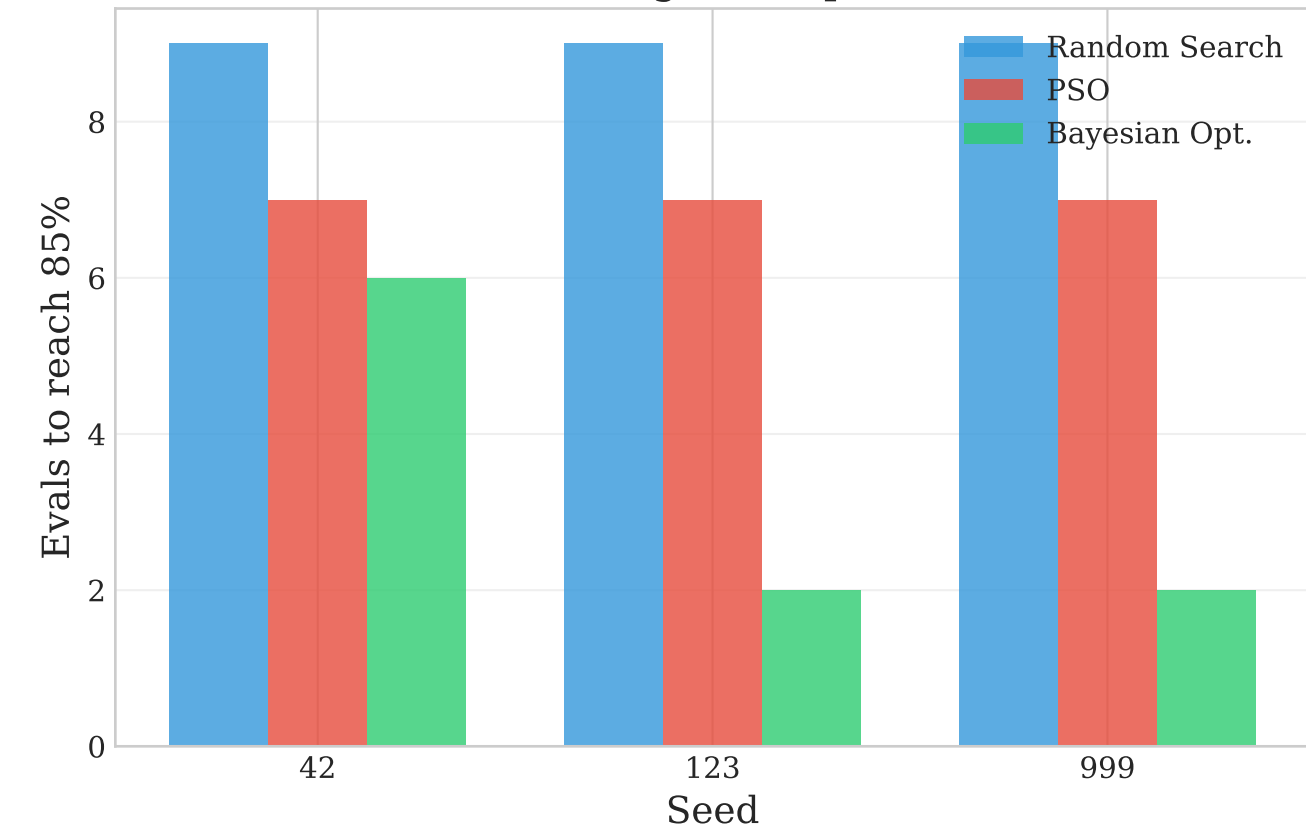
Convergence Speed
