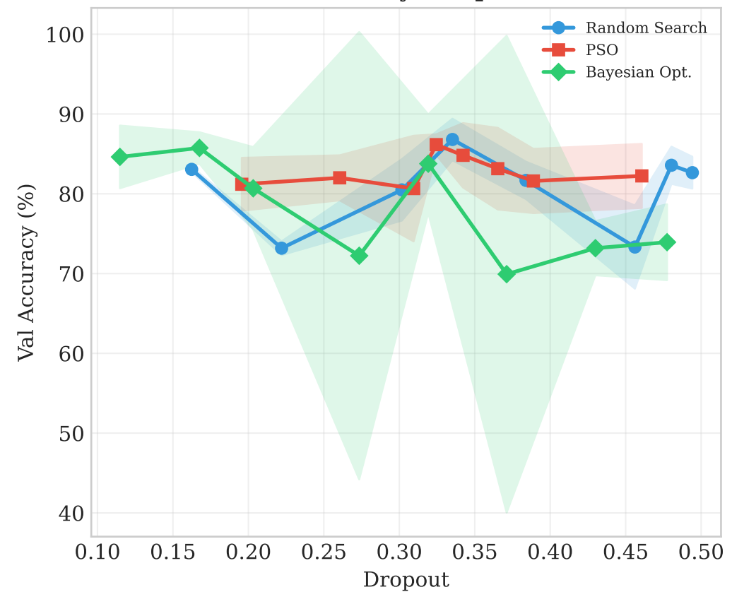
Sensitivity: Dropout
