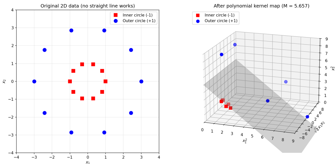
Figure 4 – The two circles in 2D (left) and after the polynomial kernel map, with the separating plane found by the SVM (right).
