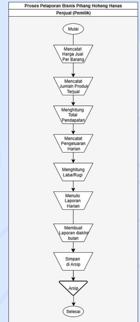
Proses Laporan
