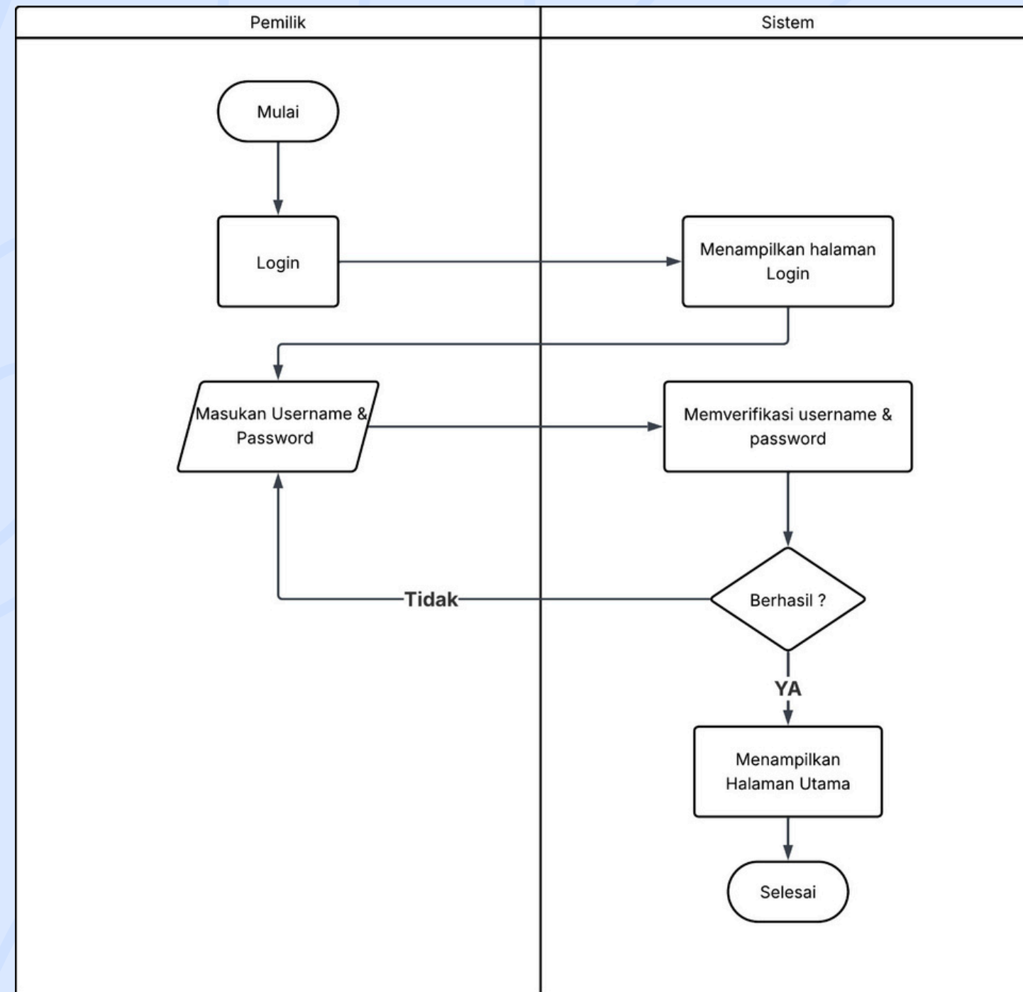
Proses Login
