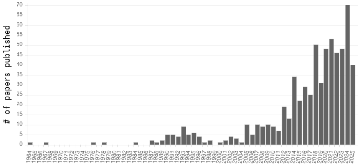
Figure 1: The number of papers published (shown on the vertical axis) regarding parallel-in-time integration has significantly, and steadily, increased over the past few decades. It is also worth noting that at the time of writing, the number of papers published this year is on track to match last year’s. Image credit [1]
