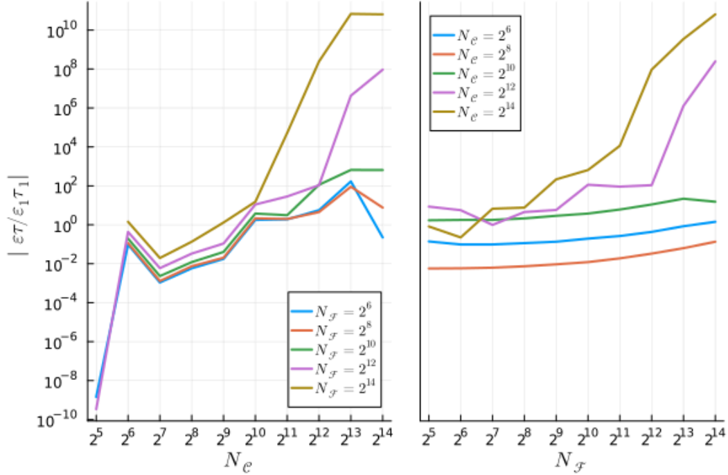
Figure 15: The efficiency of the simulation when run on a single GPU, characterized by the product of its error and runtime. This efficiency depends both on the coarse (left) and fine (right) discretizations.
