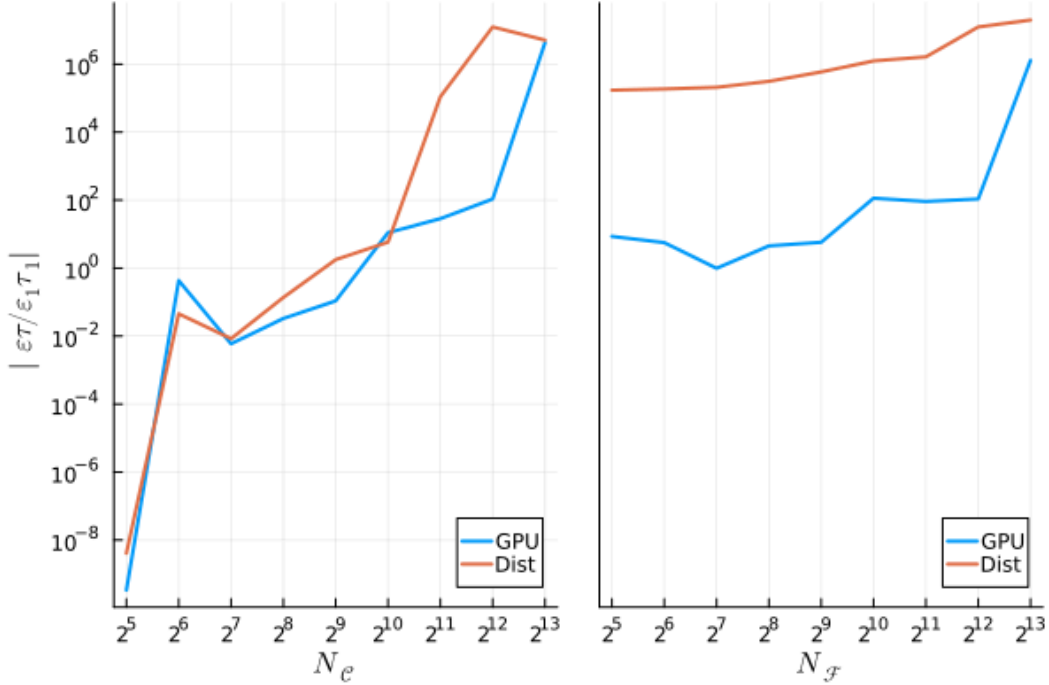
Figure 17: The efficiency of the simulation depends on the method employed. The comparison of these runtimes is shown across the range of coarse (left) and fine (right) discretizations for the a both a fine and coarse discretization of 2^{12} , respectively, chosen to highlight the differences between the methods.
