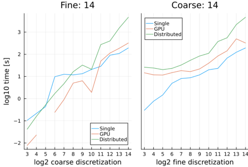
Figure 18: The runtime of the simulation depends on the method employed. The comparison of these runtimes is shown across the range of coarse (left) and fine (right) discretizations for the a both a fine and coarse discretization of 2^{14} , respectively, chosen to highlight the differences between the methods.
