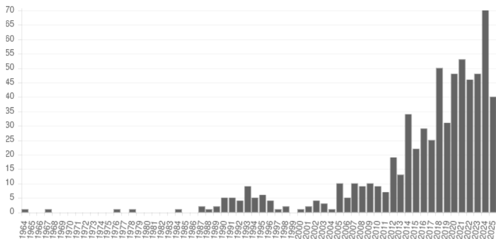
Figure 1: The number of papers published regarding parallel-in-time integration has significantly, and steadily, increased over the past few decades. It is also worth noting that at the time of writing, the number of papers published this is year is on track to match last year's. Image credit [1]
