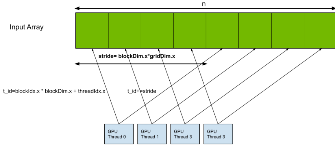
Figure 5: The indices a specific thread processes are based on how many total threads there are. Image credit [26]
