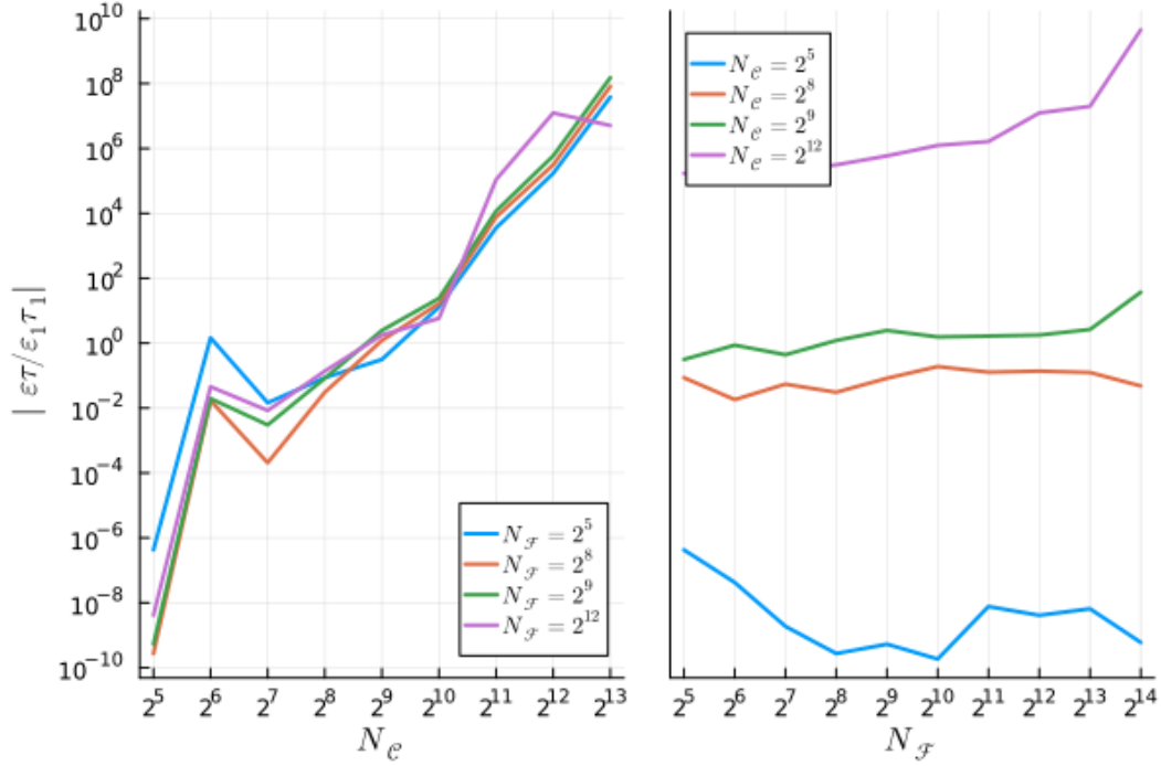
Figure 16: The efficiency of distributed simulations and how they depend on their coarse (left) and fine (right) discretizations.
