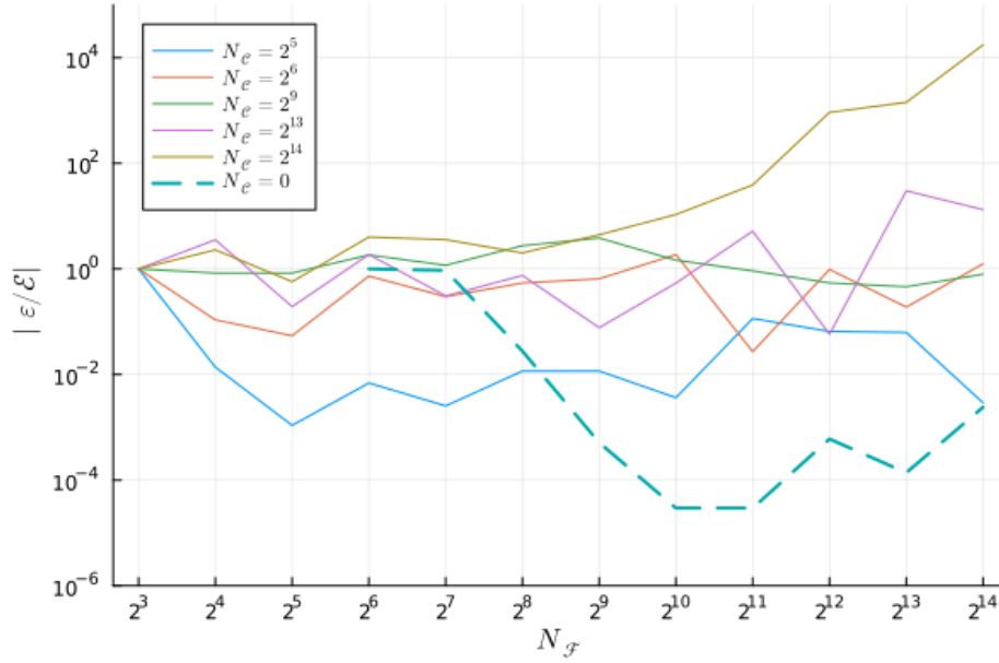
Figure 9: The absolute, normalized relative-error of the pendulum's final state for a spectrum of fine discretizations and select coarse discretizations. The error curve for a sequential evaluation (dashed N_c = 2^0 ) is included to provide a reference point.
