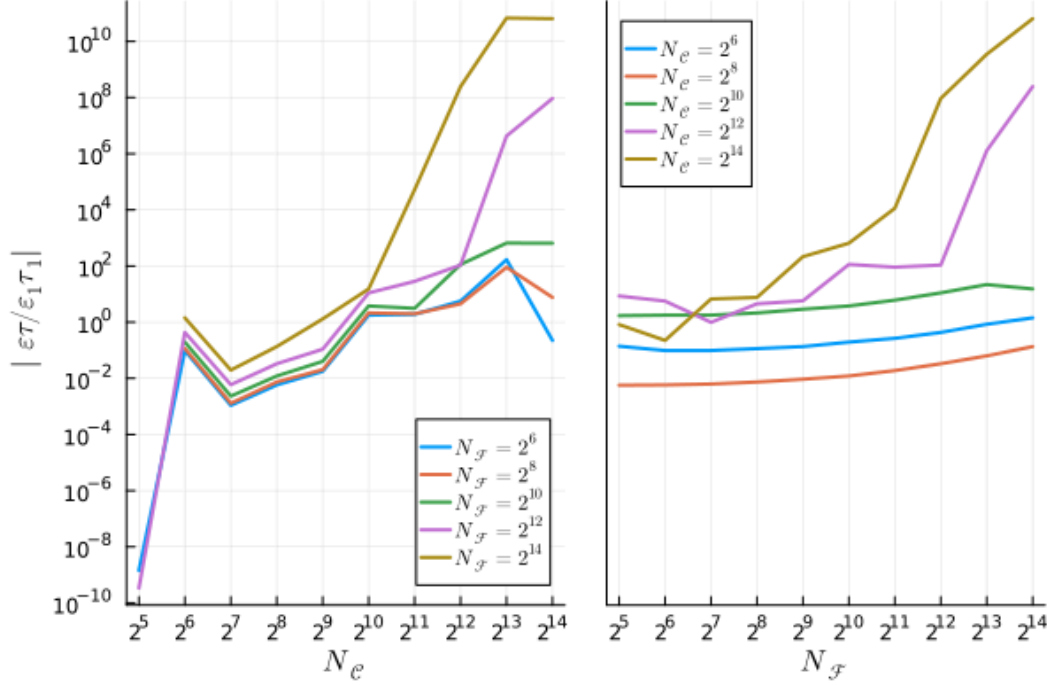
Figure 15: The efficiency of the simulation when run on a single GPU, characterized by the product of its error and runtime. This efficiency depends both on the coarse (left) and fine (right) discretizations.
