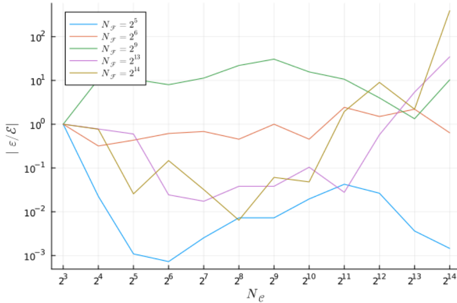
Figure 8: The absolute, normalized relative-error |\varepsilon/\mathcal{E}| of the pendulum’s final state for a spectrum of coarse discretizations and select fine discretizations. Each error \varepsilon is normalized by the error \mathcal{E} associated with the smallest coarse discretization and equal fine discretization i.e. \mathcal{E}(N_{\mathcal{F}}) = \varepsilon(2^3, N_{\mathcal{F}})
