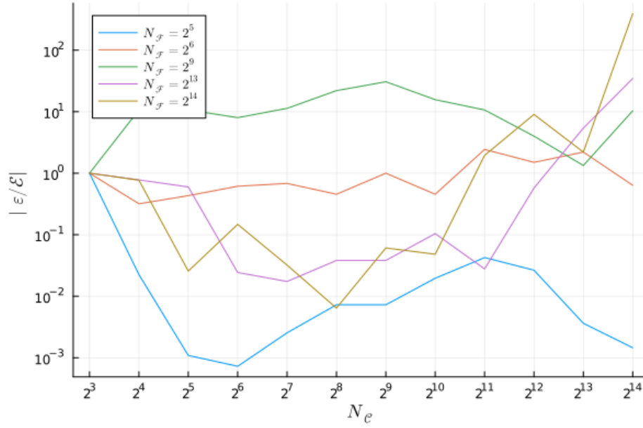
Figure 8: The absolute, normalized relative-error of the pendulum's final state for a spectrum of coarse discretizations and select fine discretizations. Each set (N_{\mathcal{F}}) of results is normalized with respect to the error \mathcal{E} when N_{\mathcal{C}} = 2^3 such that \mathcal{E} = \varepsilon(N_{\mathcal{C}} = 2^3, N_{\mathcal{F}}) .
