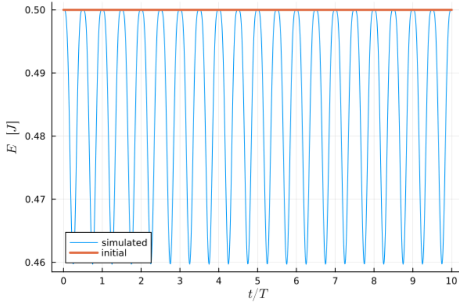
Figure 10: The stability of the simulation can be encoded in the increase of the total mechanical energy (blue) from the initial energy (orange). If the total mechanical energy does not surpass the initial energy, the simulation is stable.
