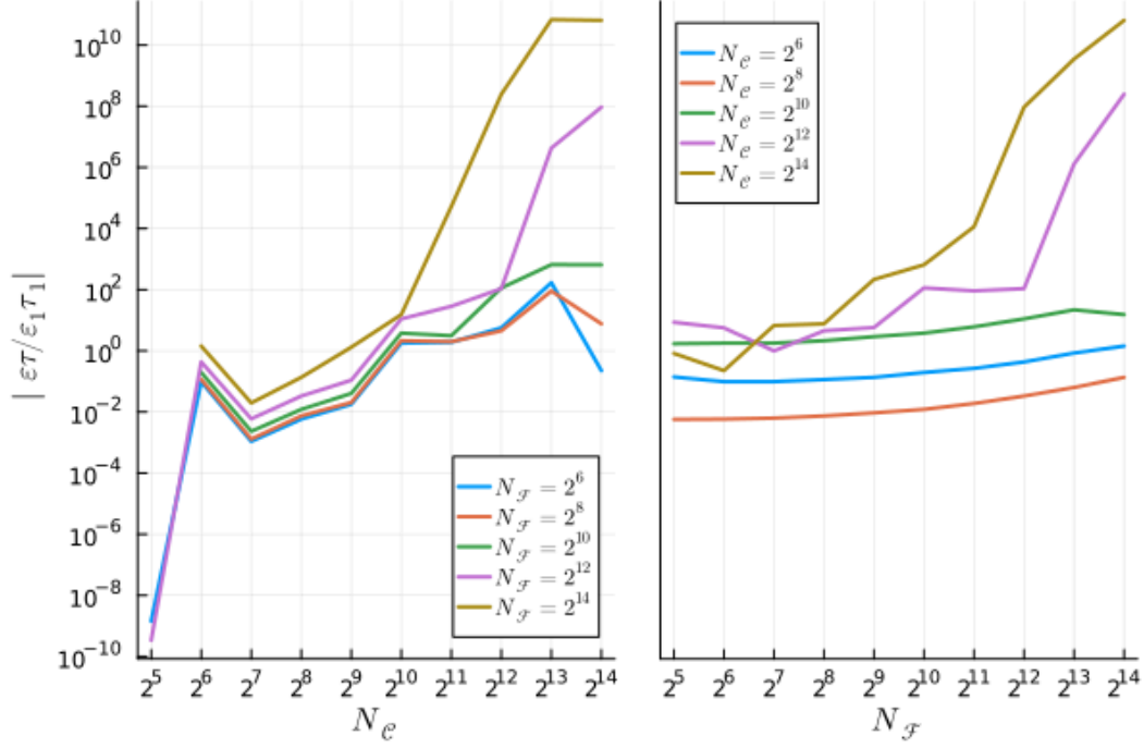
Figure 16: The efficiency of the simulation when run on a single GPU, characterized by the product of its error and runtime. This efficiency depends both on the coarse (left) and fine (right) discretizations.
