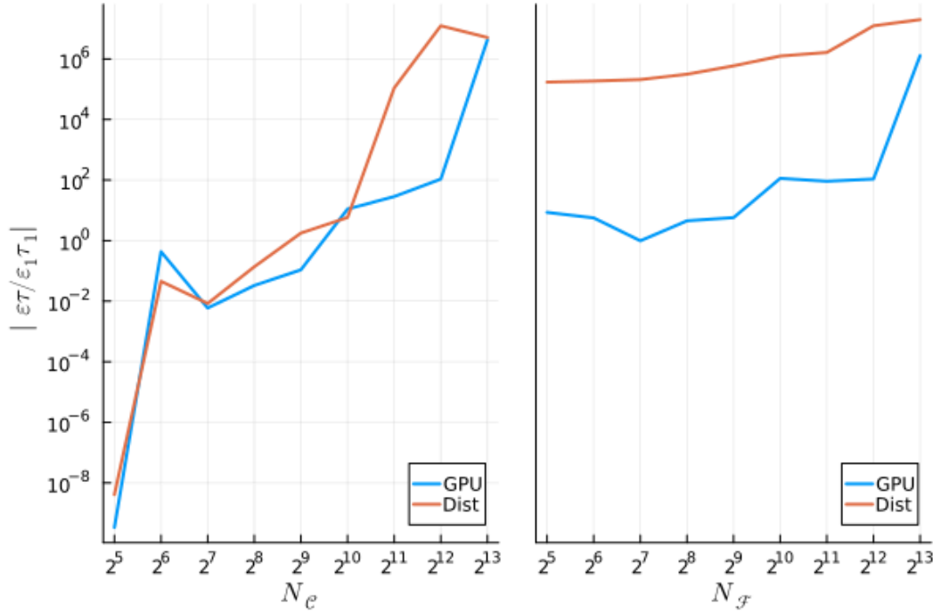
Figure 18: The efficiency of the simulation depends on the method employed. The comparison of these runtimes is shown across the range of coarse (left) and fine (right) discretizations for the a both a fine and coarse discretization of 2^{12} , respectively, chosen to highlight the differences between the methods.
