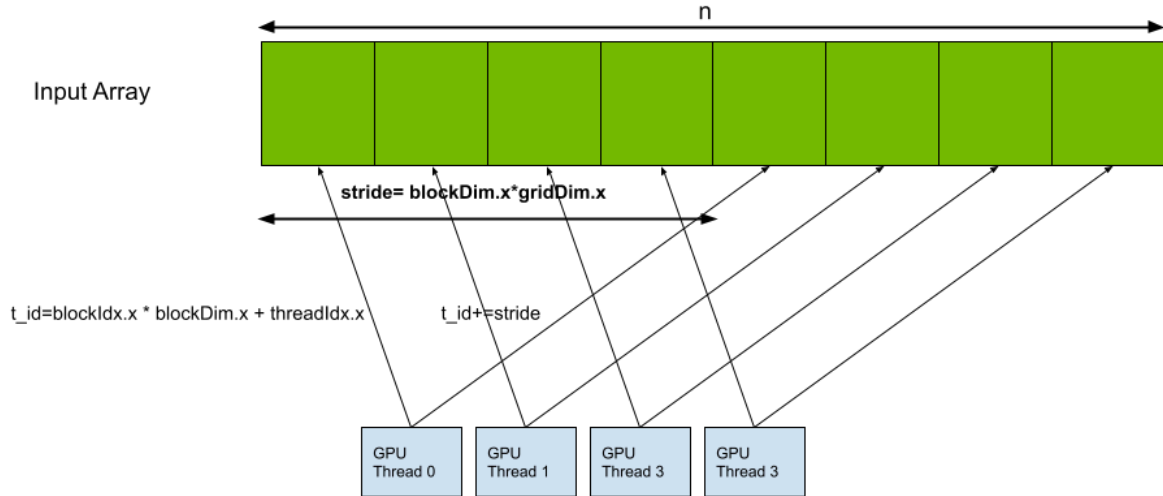
Figure 5: The indices a specific thread processes are based on how many total threads there are. Image credit [3]
