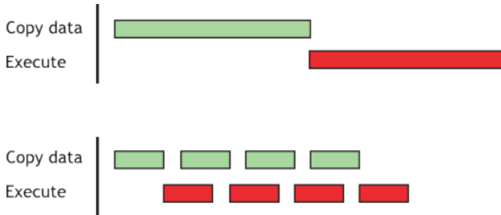
Figure 12: When only using pinned memory, all data needs to be copied from the host to the device before any computation can begin (top). Using zero-copy memory (bottom) allows for data transfers to happen at the same time as computation. Sourced from [30].
