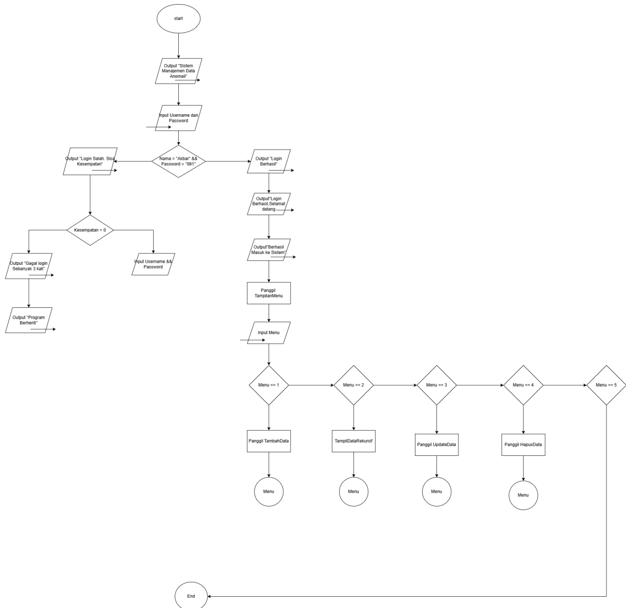
Gambar 1.1 Flowchart
