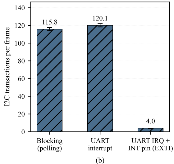
Fig. 1. Per-frame latency of the VL53L8CX-to-STM32F411RE link under three driver configurations. (a) Latency breakdown; (b) number of I 2 C transactions per frame. Error bars show \pm 1 SD. 8 \times 8 resolution at 15 Hz, I 2 C 400 kHz, CPU 84 MHz, n = 7986 frames.
