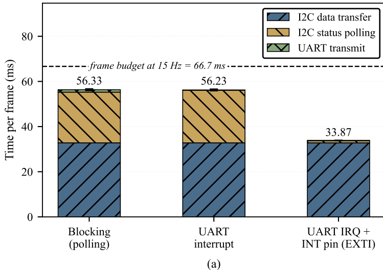
Fig. 1. Per-frame latency of the VL53L8CX-to-STM32F411RE link under three driver configurations. (a) Latency breakdown; (b) number of I 2 C transactions per frame. Error bars show \pm 1 SD. 8 \times 8 resolution at 15 Hz, I 2 C 400 kHz, CPU 84 MHz, n = 7986 frames.
