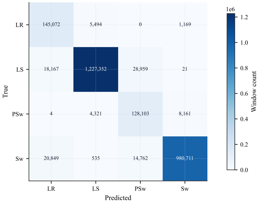
FP32 | Test (6 subjects) Accuracy 96.04%
