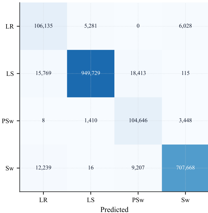
FP32 | Validation (8 subjects) Accuracy 96.29%
