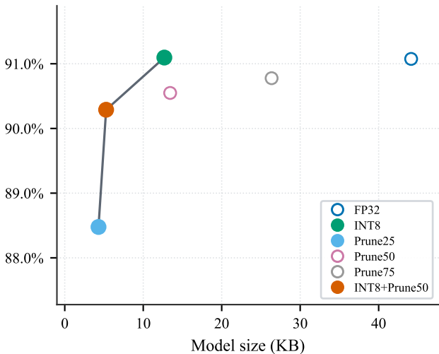
Macro F1-score
