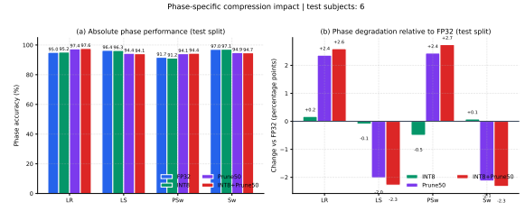
Fig. 3. Phase-specific accuracy change relative to the FP32 baseline under compression.
