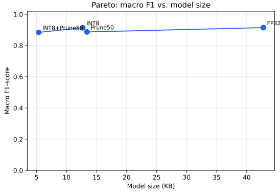
Fig. 2. Pareto front: macro F1-score vs. estimated deployment size (KB) for FP32, INT8, Prune50, and INT8+Prune50.
