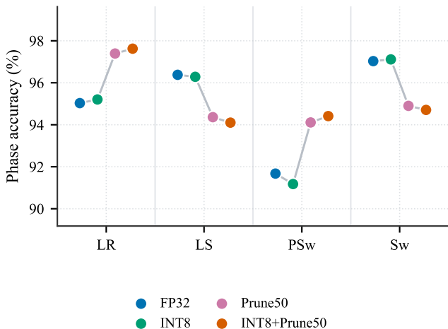
(a) Absolute phase performance
