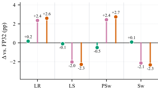
(b) Degradation relative to FP32
