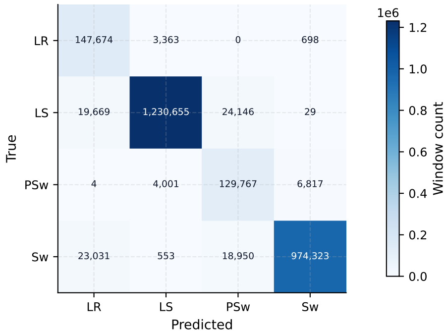
FP32 | Validation (5 subjects) Confusion matrices by compression config and evaluation fold Accuracy 95.89%
