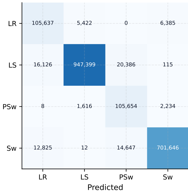
FP32 | Validation (5 subjects) Confusion matrices by compression config and evaluation fold Accuracy 95.89%
