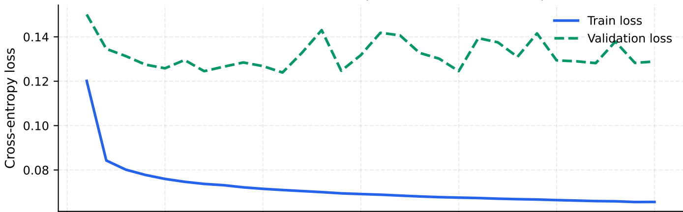
(a) Loss curves (Train (24 subjects) / Validation (5 subjects))
