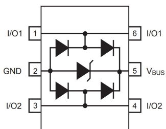
Functional diagram (top view)
