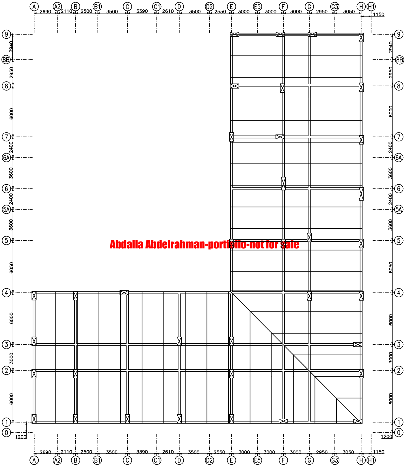
FLOOR KEY PLAN: RB ( Rooftop & Truss Spacing )
