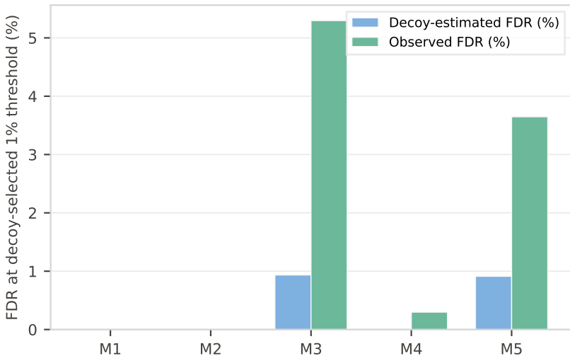
Decoy vs observed FDR
