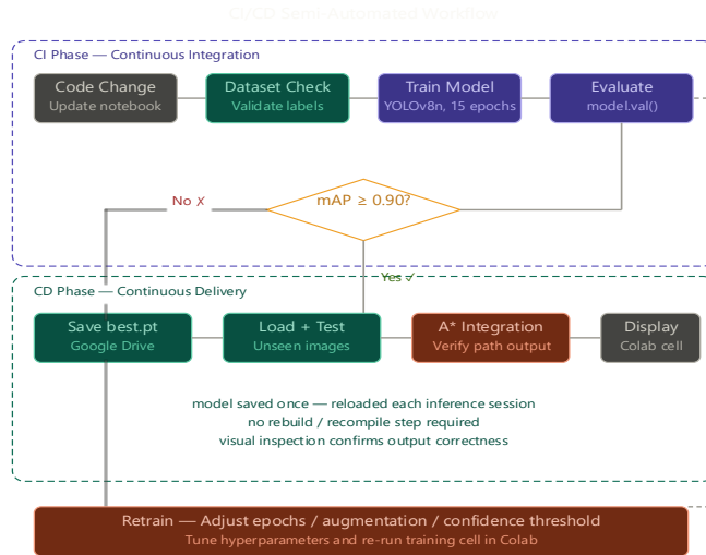
Figure 3.9: CI/CD Workflow
