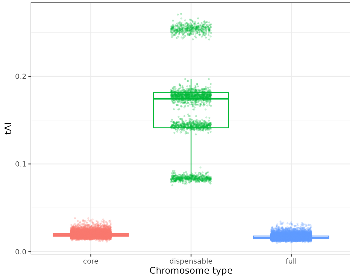
tAI distribution across chromosome types
