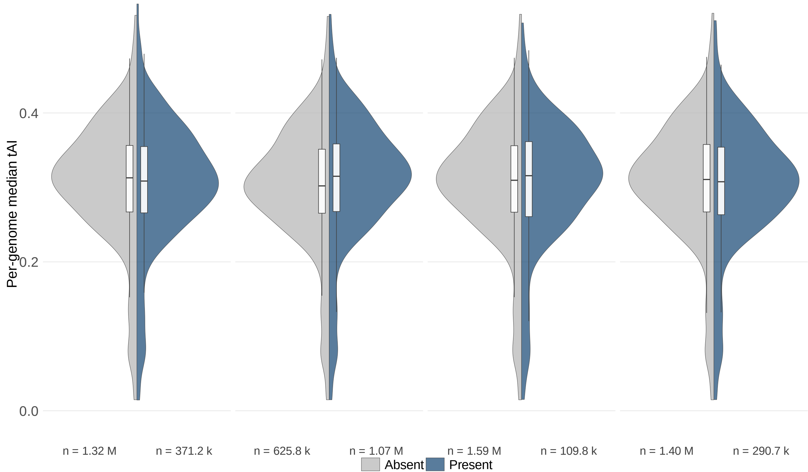
Signal peptide
