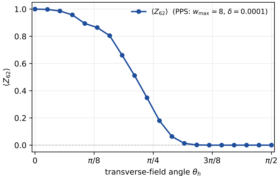
127-qubit kicked Ising ( \text{RZZ}(-\pi/2) , 20 Trotter steps, IBM Eagle heavy-hex)
