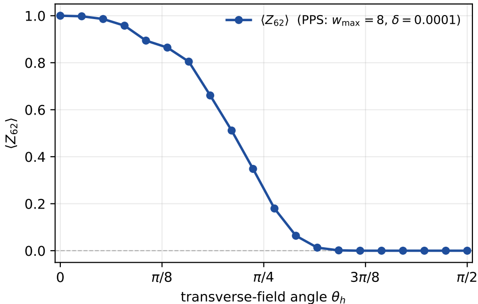
127-qubit kicked Ising (RZZ( -\pi/2 ), 20 Trotter steps, IBM Eagle heavy-hex)
