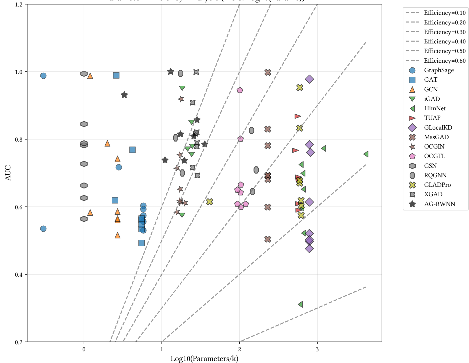
Parameter Efficiency Analysis (AUC/Log10(Params))
