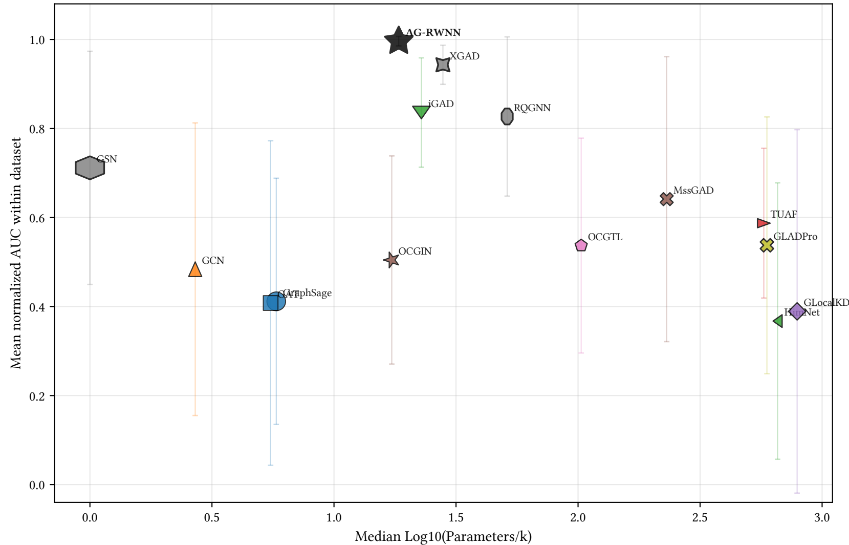
Cross-dataset parameter-performance tradeoff
