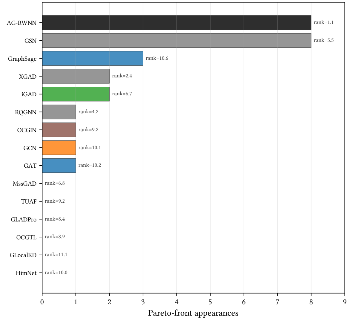
How often each model is Pareto-efficient
