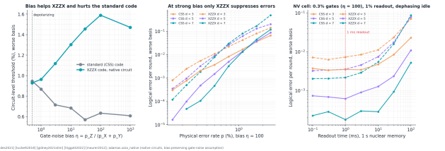
Figure 5: Native XZZX circuits with biased gate noise: thresholds versus bias, logical error at \eta = 100 , and the NV readout scenario.
