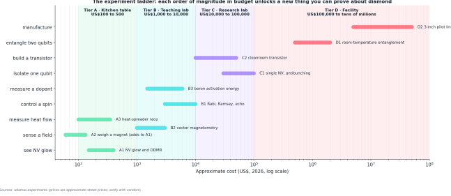
Figure 7: Ten experiments in four budgets, with parts, steps, safety, and simulated expected results; a firmware kit makes the US$150 to 400 ODMR experiment runnable.
