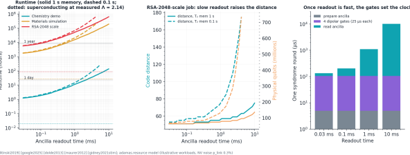
Figure 6: Resource estimate from the circuit-level fits: runtime, code distance, and the composition of one syndrome round.
