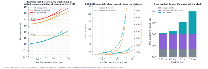
Figure 5: Resource estimate from the circuit-level fits: run-time, code distance, and the composition of one syndrome read.
