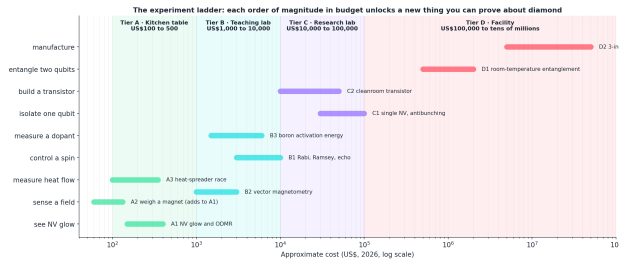
Figure 6: Ten experiments in four budgets, with parts, steps, safety, and simulated expected results; a firmware kit makes the US$150 to 400 ODMR experiment runnable.
