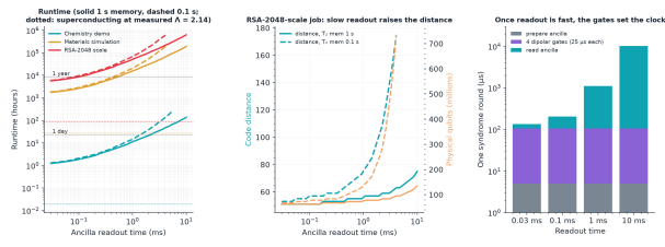
Figure 6: Resource estimate from the circuit-level fits: run-time, code distance, and the composition of one syndrome round.
