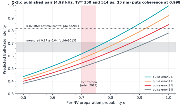
Figure 3: Echoed NV-NV gate budget evaluated with the published pair [16]: fidelity versus charge-state preparation probability. Coherence limits fidelity to 0.998.
