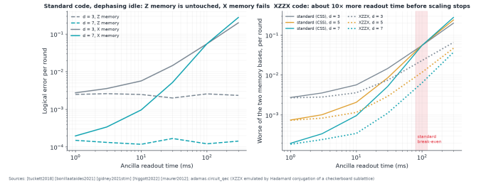
Figure 4: Circuit-level surface code with dephasing idle errors during readout. Left: standard code, Z and X memories. Right: worse basis for standard and XZZX codes.
