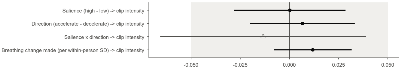
Correlations (r)
