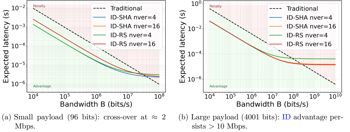
Figure 5.2: End-to-end latency vs. channel bandwidth ( p_{desync} = 0.1 ). The plots reveal the break-even point where the computational cost of ID ( t_{ver} ) intersects with the transmission cost of the baseline. In the low-bandwidth regime ( B < 1 Mbps), ID offers up to 10\times latency reduction.
