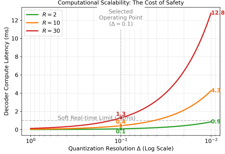
Figure 4.4: Computational scalability analysis showing decoder latency as a function of quantization resolution \Delta . The red curve represents the safe-harbor configuration ( R = 30 ). At the high-precision limit ( \Delta = 0.01 ), latency reaches a prohibitive 12.8 ms. However, at the selected operating point ( \Delta = 0.1 , indicated by the vertical dotted line), the latency drops to approximately 1.3 ms, balancing maximum physical coverage with real-time computational feasibility.
