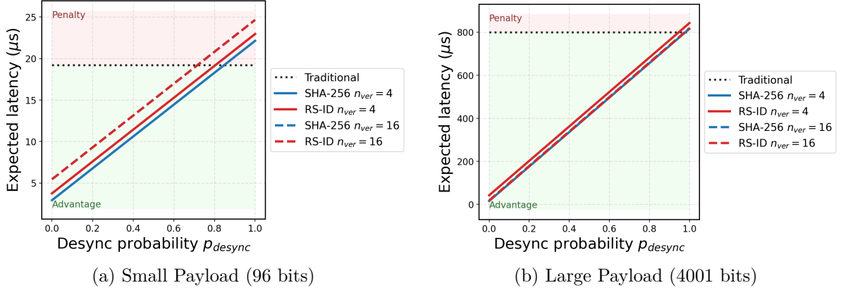
Figure 5.3: Latency sensitivity to prediction error ( B = 5 Mbps). The intersection with the traditional baseline indicates the p_{desync} range in which ID -based synchronization yields lower expected latency. For 4001-bit payloads (b) the cross-over shifts closer to p_{desync} = 1 compared to the 96-bit payloads (a).
