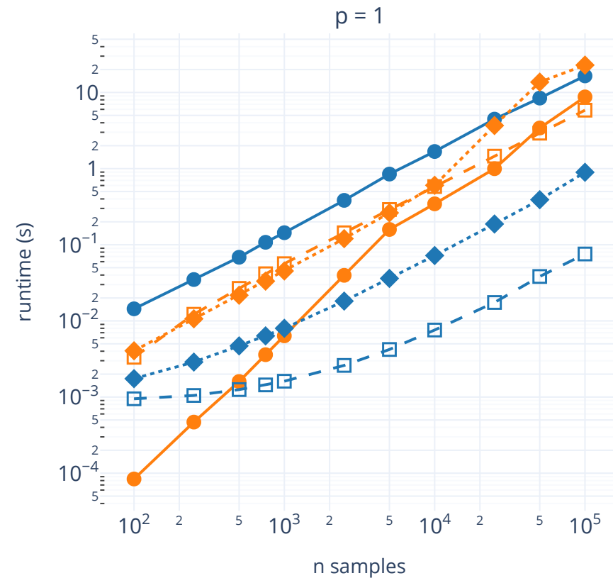
Change-in-mean benchmark (L2 cost): runtime vs. sample size Legend column = package, line style + marker = search algorithm. Best of N runs, fit + predict.
