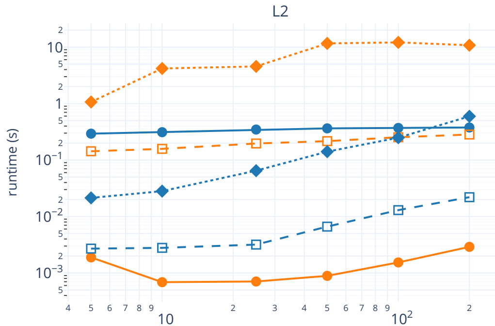
Multivariate change detection benchmark (n = 2000): runtime vs. dimension Legend column = package, line style + marker = search algorithm. Best of N runs, fit + predict. ESAC is skchange-only.
