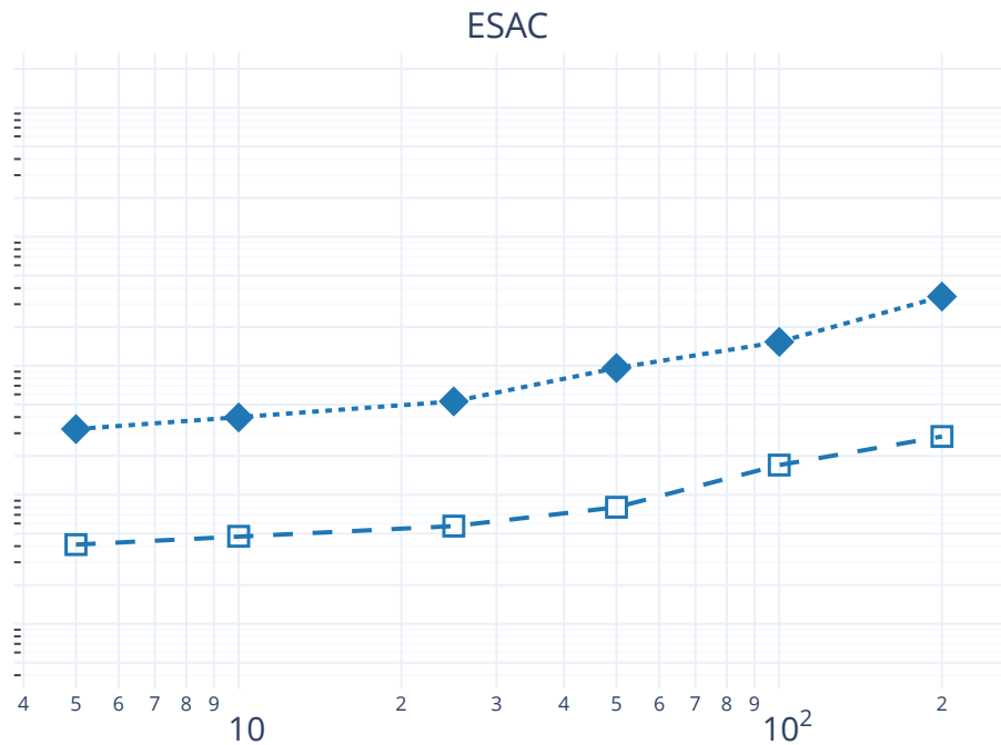
Multivariate change detection benchmark (n = 2000): runtime vs. dimension Legend column = package, line style + marker = search algorithm. Best of N runs, fit + predict. ESAC is skchange-only.
