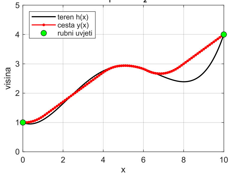
slučaj A, N = 100 ( b_1 = 0.5 , b_2 = 0.5 ), J = 19.659
