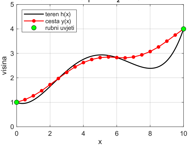
slučaj B, N = 20 ( b_1 = 0.5 , b_2 = 0.2 ), J = 4.907
