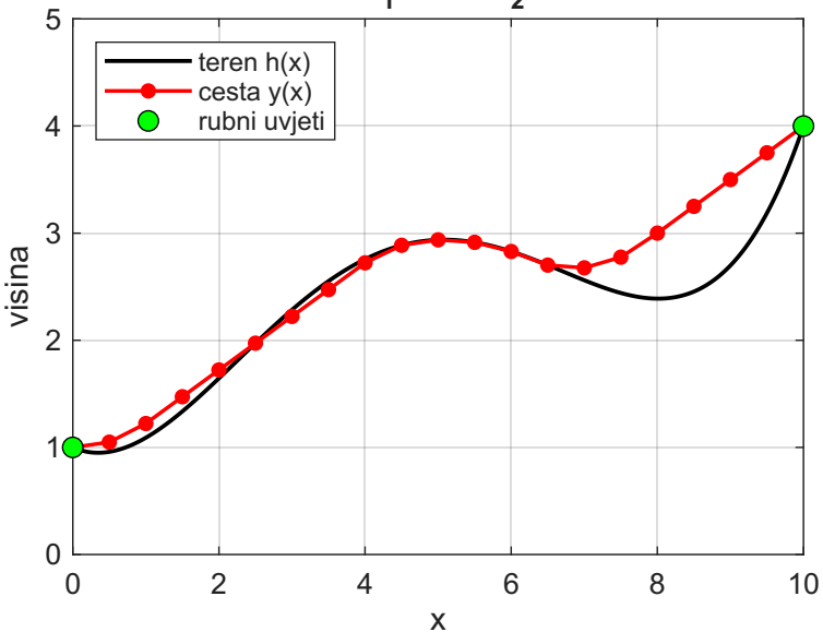
slučaj A, N = 20 ( b_1 = 0.5 , b_2 = 0.5 ), J = 3.832
