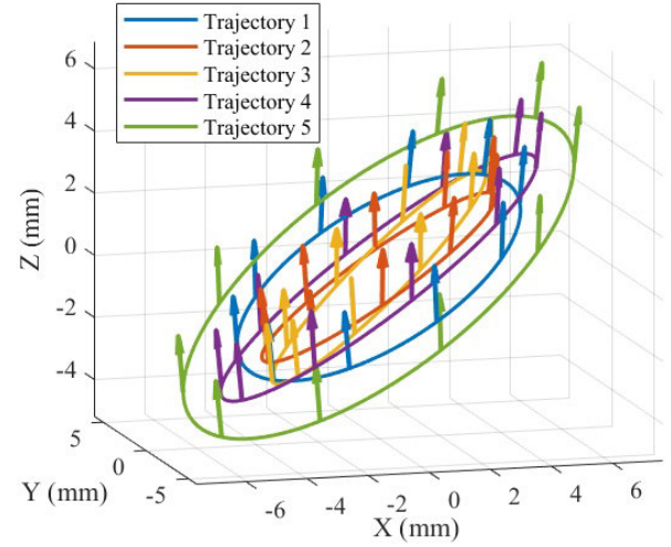
Fig. 5. Five motion trajectories of the phantom in the test set, with arrows indicating the directions at the sampled points.
