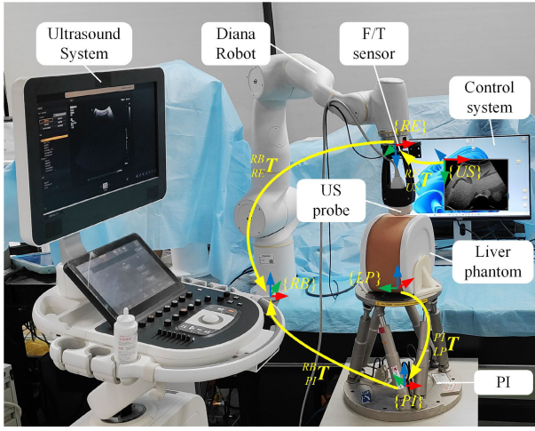
Fig. 4. Experimental setup for robotic respiratory liver motion compensation.
