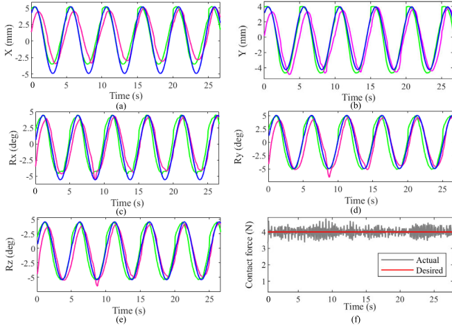
Fig. 6. Visualization results of robotic respiratory liver motion compensation for (a) translation along the X-axis, (b) translation along the Y-axis, (c) rotation around the X-axis, (d) rotation around the Y-axis, (e) rotation around the Z-axis, and (f) contact force in the Z-axis direction. In (a)–(e), pink curves illustrate robotic respiratory liver motion compensation results, the green curves show the estimation results using our ReME-Net, while the blue curves represent the given liver motion. For ease of comparison, all data in (a)–(e) have been mean-centered.
