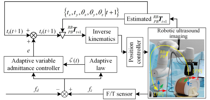
Fig. 3. Block diagram of the hybrid force–position control method.
