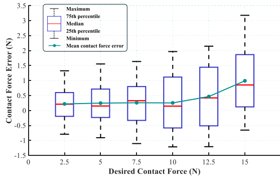
Fig. 9. Force tracking performance at various desired contact force.
