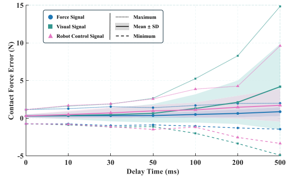
Fig. 8. Impact of visual, force, and robot control signal latency on contact force tracking performance of the proposed motion control framework.
