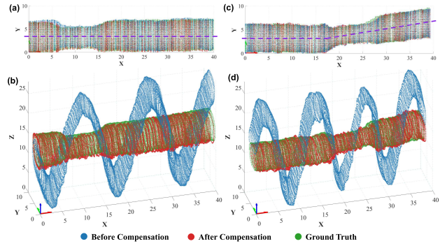
Fig. 10. (a) and (b) Performance of the 3-D US imaging compensation framework on a straight-line vessel. (c) and (d) Polyline vessel mimicking a human vascular bifurcation.
