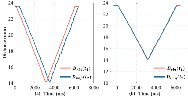
Fig. 5. Temporal calibration results. The red line represents distance from robot forward kinematics and the blue line represents distance from US images and spatial calibration. (a) Results before temporal mismatch compensation. (b) Results after temporal mismatch compensation.
