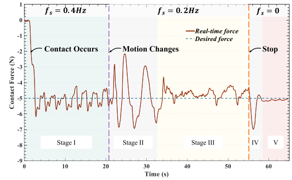
Fig. 7. Contact force tracking performance of the proposed motion control framework under respiratory frequency changes.
