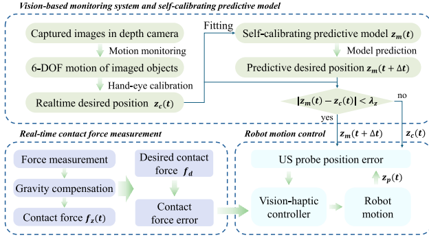
Fig. 3. Our proposed vision-haptic fusion motion control framework, including vision-based motion monitoring system, self-calibrating predictive model, real-time contact force measurement, and robot motion control.
