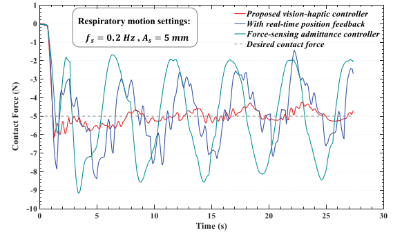
Fig. 6. Performance of the contact force tracking under respiratory motion ( f_s = 0.2 Hz and A_s = 5 mm). The proposed vision-haptic fusion motion controller with predictive position feedback (red line). Admittance controller with real-time position feedback (blue line). Admittance controller [11] with only force sensing (green line).
