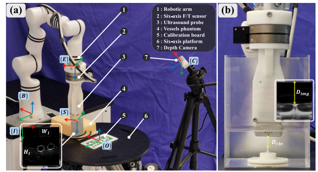
Fig. 2. (a) System setup and coordinate definition. (b) Temporal calibration system setup.
