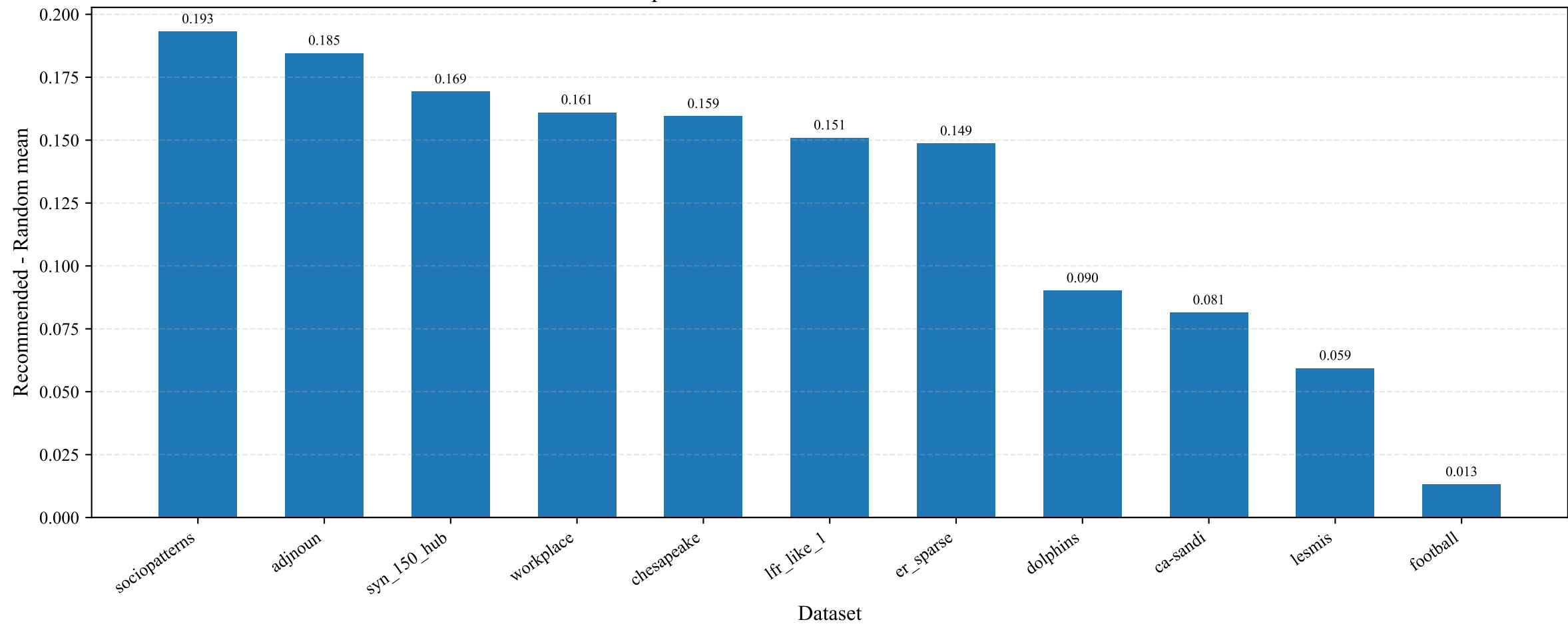
Improvement over Random Search Mean
