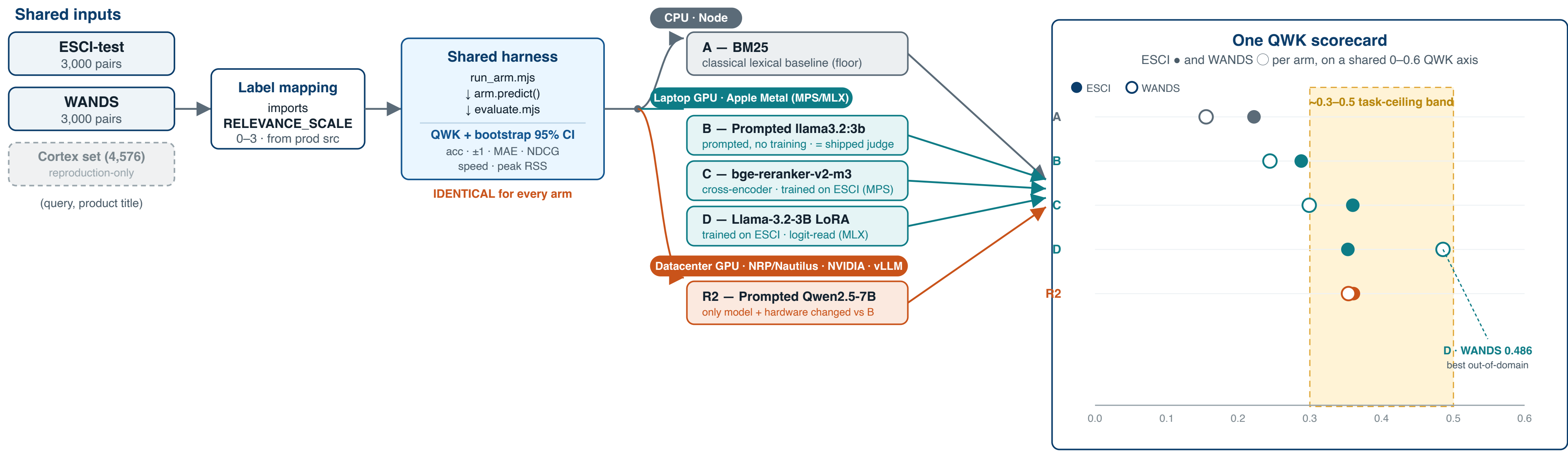
Figure 1. One shared evaluation pipeline fanning across three hardware tiers — CPU, laptop GPU (Apple Metal), datacenter GPU (NRP/Nautilus · vLLM) — all converging on a single QWK scorecard. The harness box is byte-identical for every arm , so any movement is attributable to the model & hardware, not pipeline drift. Vector diagram (built for print). Every plotted QWK is the exact value from the results table below.
