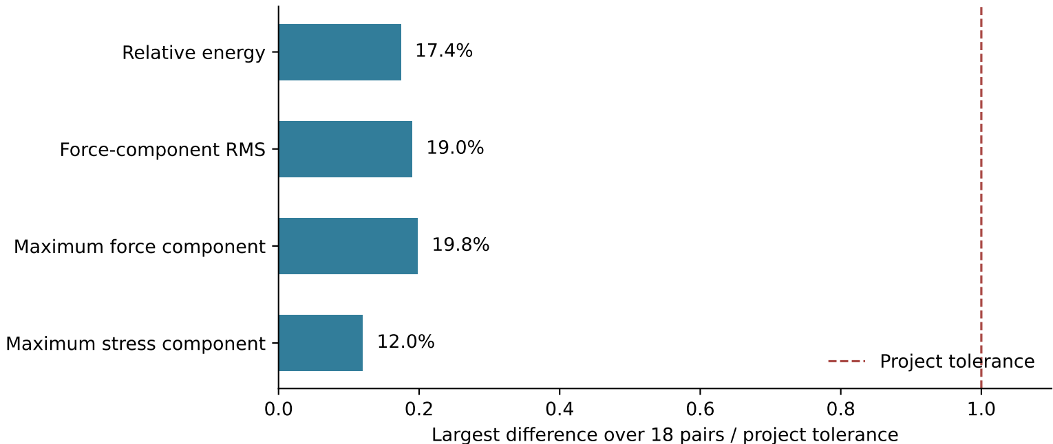
k6 versus k7 at 600 eV: all 18 pairs pass all four budgets
