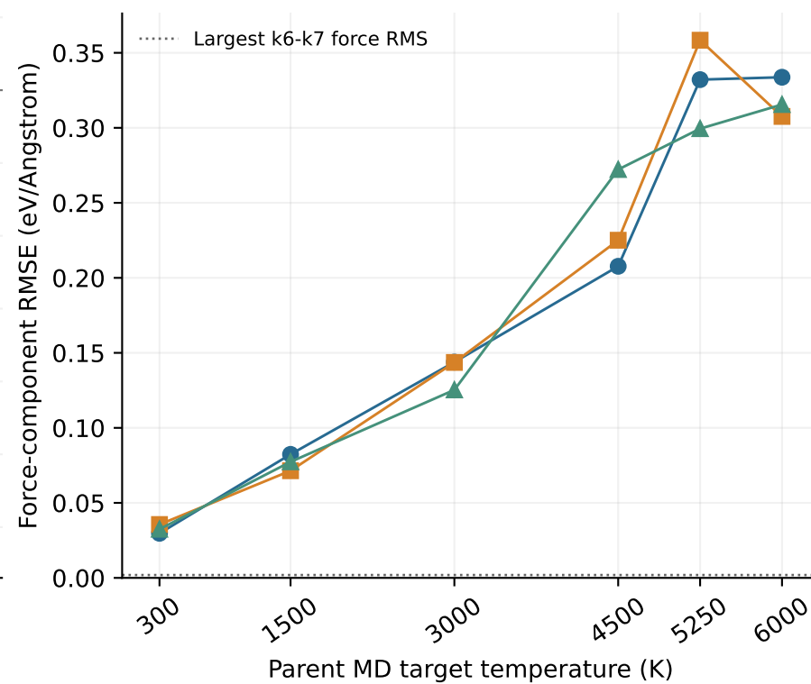
Force error
