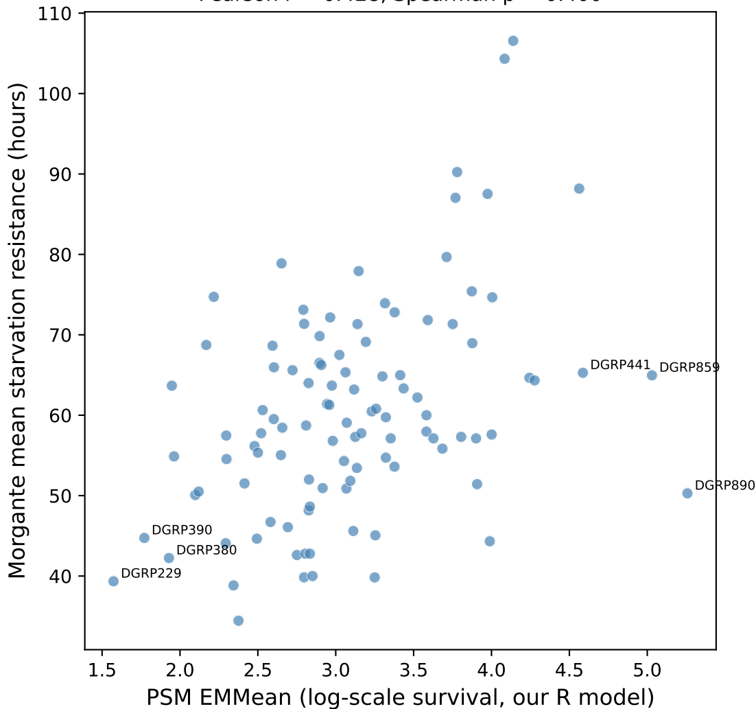
EMMeans vs Morgante et al. 2015 (n=104 lines) Pearson r = 0.428 , Spearman \rho = 0.400
